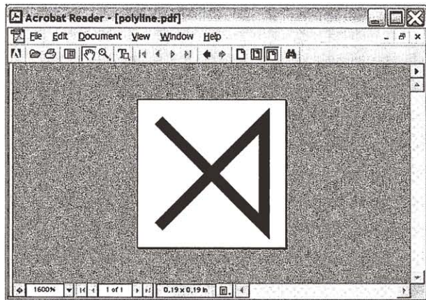
图21-2 PolyLine([(0, 0), (10, 0), (10, 10), (0, 10)])
