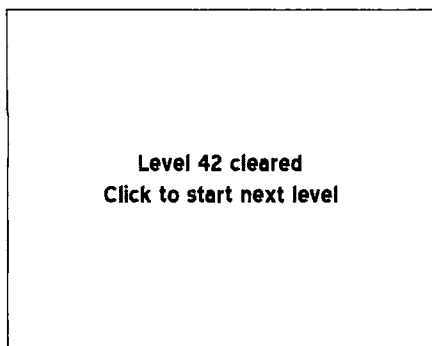
图29-5 “过关”屏幕
