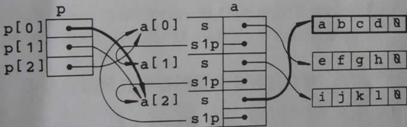
(c) *(++(p[0])) . s
